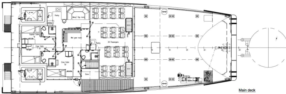
Main deck
