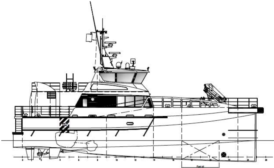
Profile
